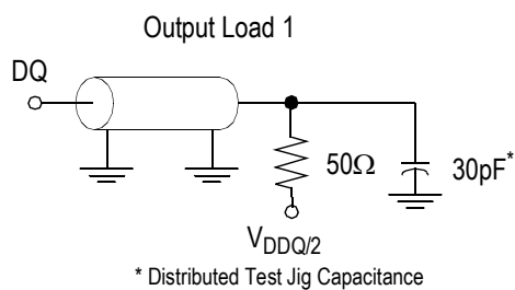
Figure 1: Output Loading
